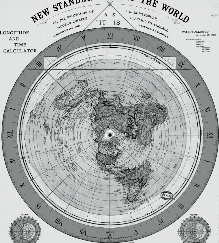
JUNE SOLSTICE.
